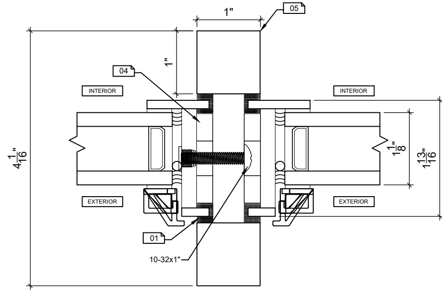
701 / MULLION DETAIL-FIXED TO FIXED
