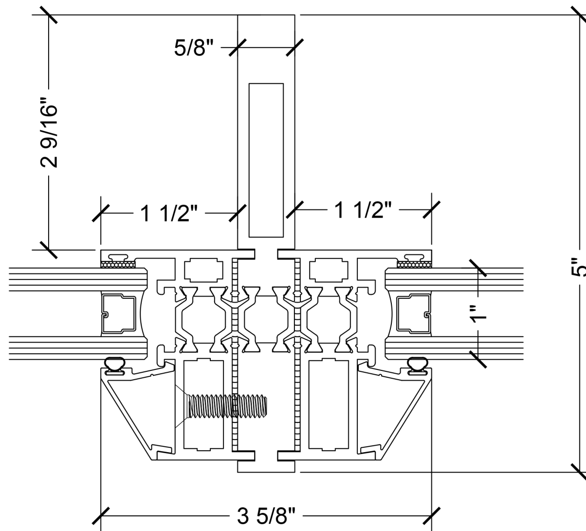
5" thermal mull assembly
