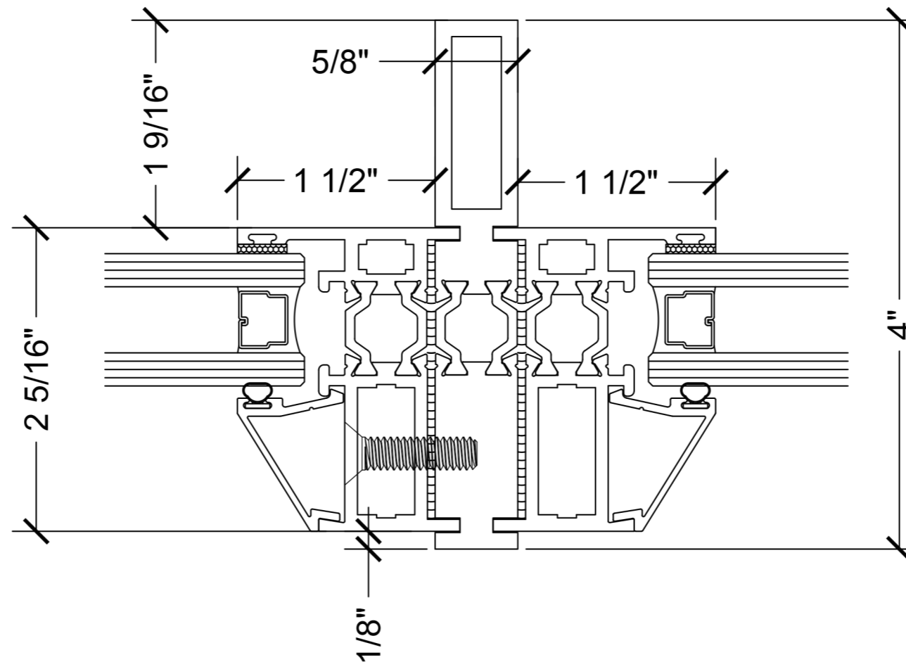
4" thermal mull assembly
